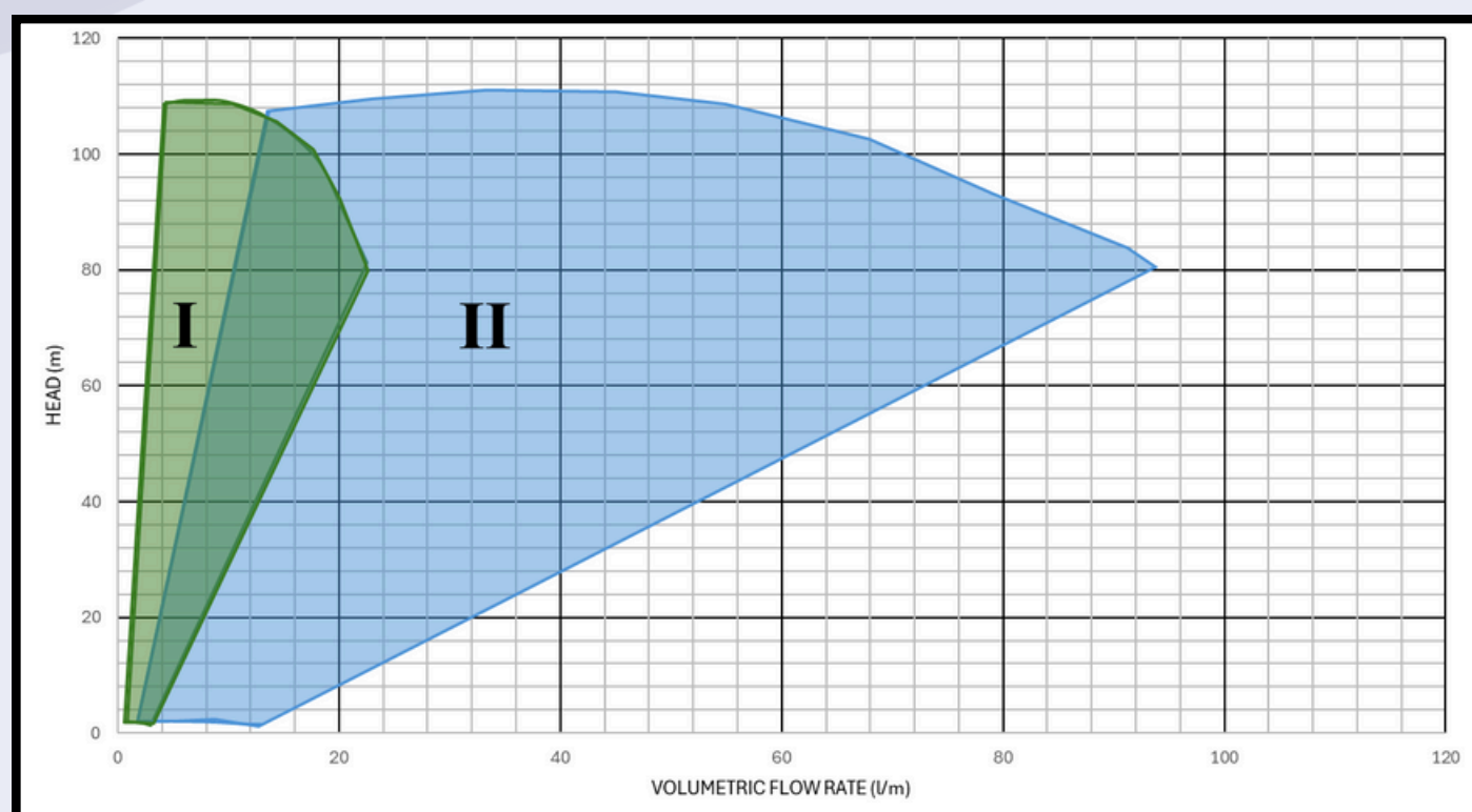
Pump Performance Map
